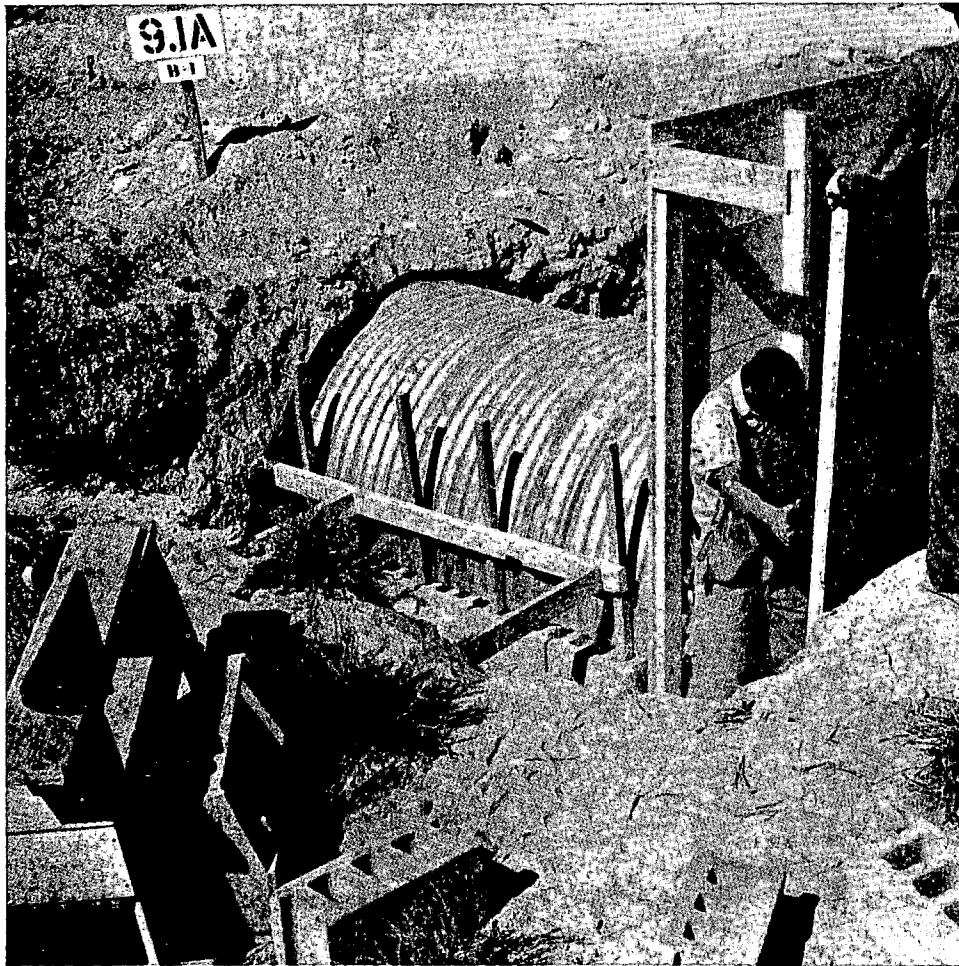
Fig. 3—Metal-arch shelter B-1 under construction.
